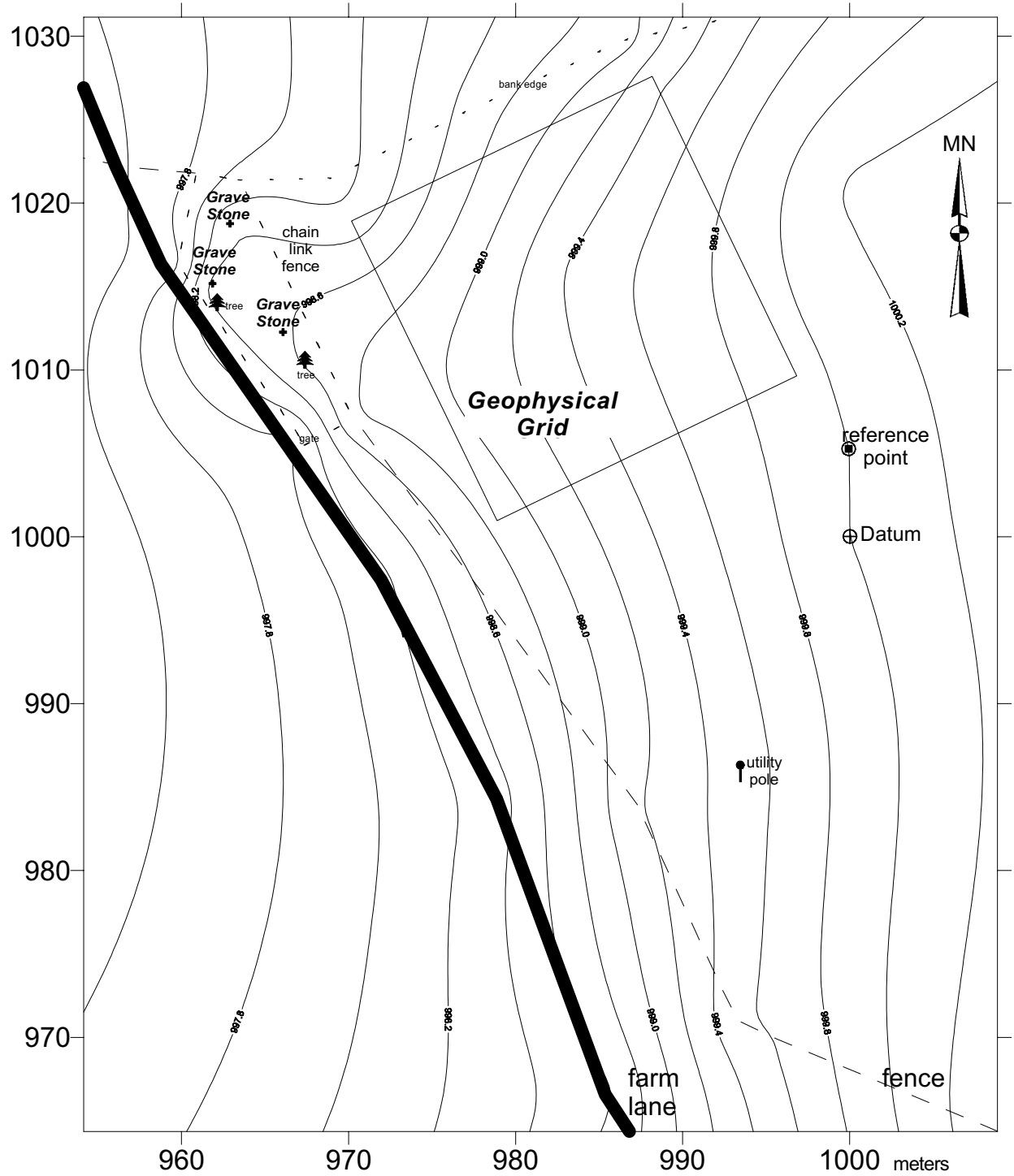
Figure 17. Geophysical grid at Site 14PO312, or the 49ers Cemetery, on the Jim Tessendorf farm, November 14, 2000, and August 1, 2001. Axes are scaled in meters; the contour interval is 0.2 m.
