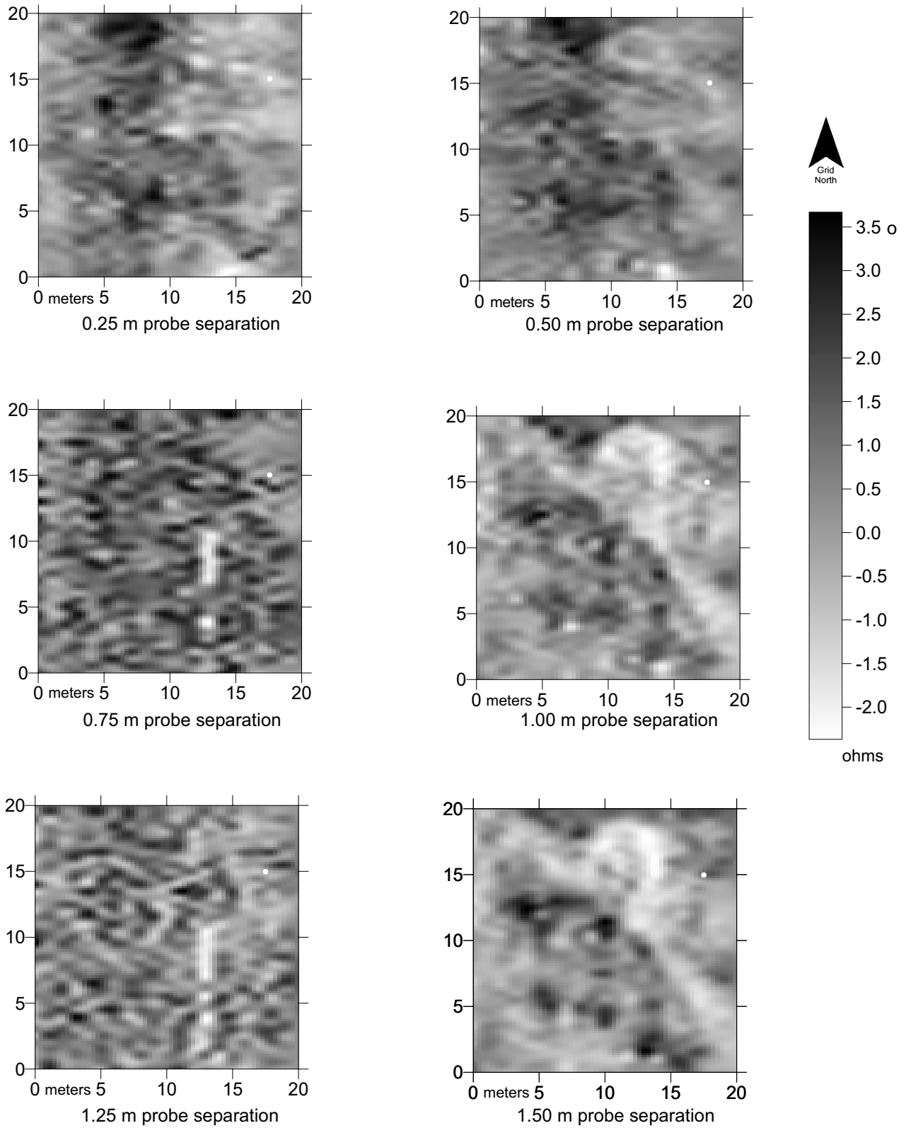
Figure 51. Image map of multiplexed soil resistance data from Site 14MH323. Axes are scaled in meters; the white dot represents marked gravestone.
