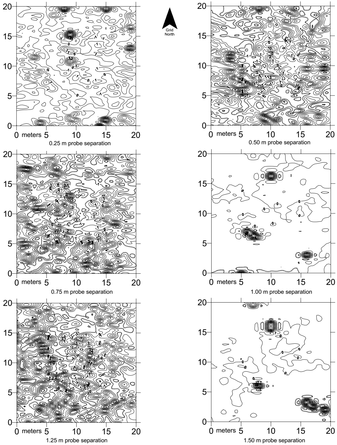
Figure 54. Contour map of multiplexed soil resistance data from Site 14PO312, August 1, 2001. Axes are scaled in meters; the contour interval is 0.5 ohms.
